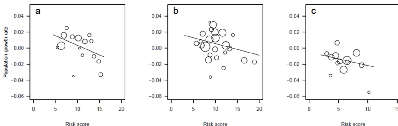
Figure 1. The relationship between risk score (with no scaling mechanism) and annual population growth rate of 52 forest bird species. Species with different migration strategies are presented separately: a) non-migratory ( y = -0.002x + 0.03 , r^2 = 0.29 ); b) within Europe migrants ( y = -0.001x + 0.02 , r^2 = 0.09 ); c) wintering outside Europe ( y = -0.002x - 0.005 , r^2 = 0.07 ). The sizes of data points are proportional to the standard error of population growth rate estimate, with larger points having smaller standard error and thus greater weight in models. Relationships were tested concurrently with migration strategy as a separate term in the model ( P = 0.01 , see text for details). doi:10.1371/journal.pone.0064552.g001
